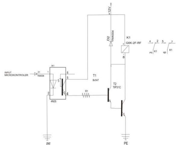
Gambar 6. Rangkaian Centrallock
