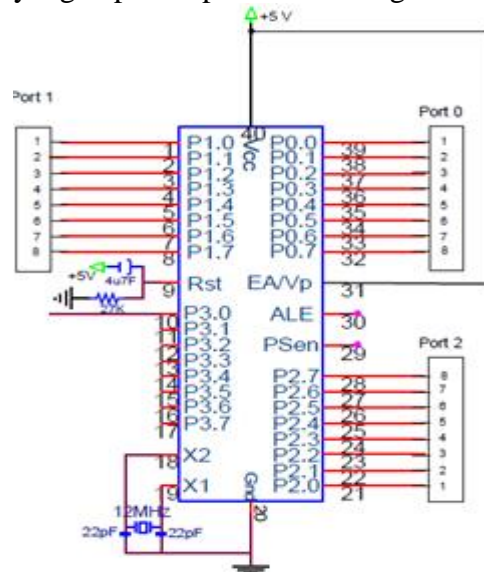
Gambar 4. Sistem Minimum
